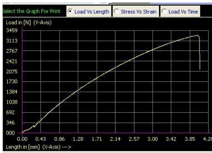
Fig. 4: Load Vs deflection curve (GSGBG)
